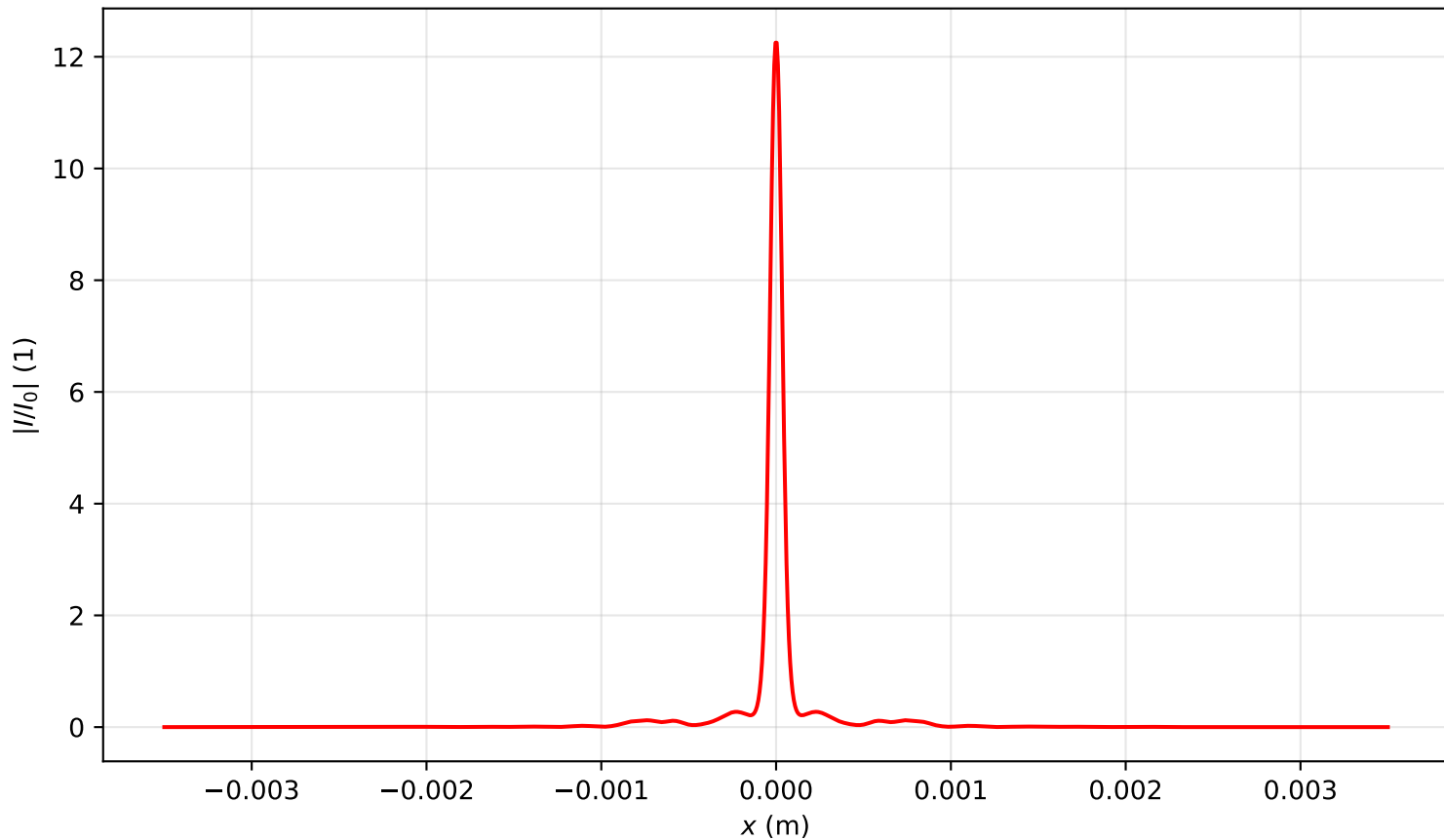
Intensity profile I(x, y = 0, z = 1.194)/I_0 , P_{in}=8.0P_{cr} , artificial time
